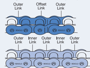
To lengthen an even link chain by one pitch
