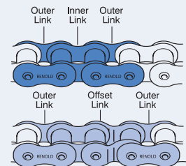
To lengthen an even link chain by one pitch
