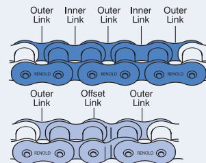
To shorten an even link chain by one pitch
